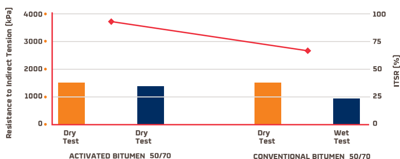
Water sensitivity test results (UNE-EN 12697-12) [AC22 G mix, with Porphyry Aggregate and 4.1 % of bitumen 50/70 s/a]
