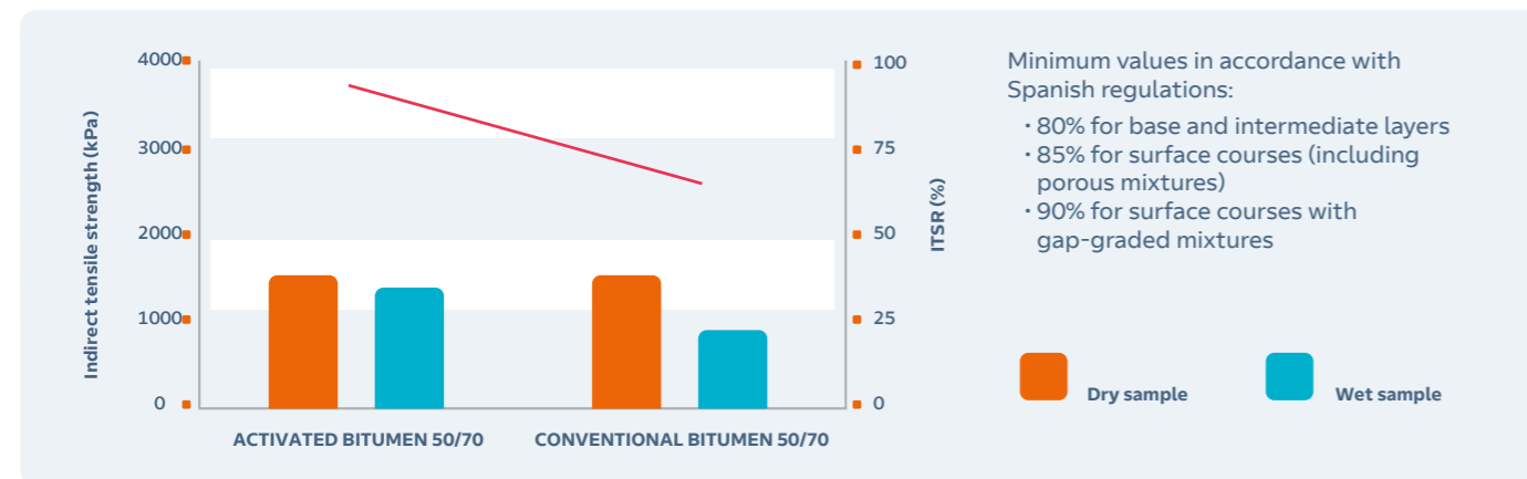
Water sensitivity test results (EN 12697-12) (AC22G mixture, with a porphyry aggregate and 4.1% bitumen 50/70 without additives). These values are illustrative and not binding, nor subject to specification.
